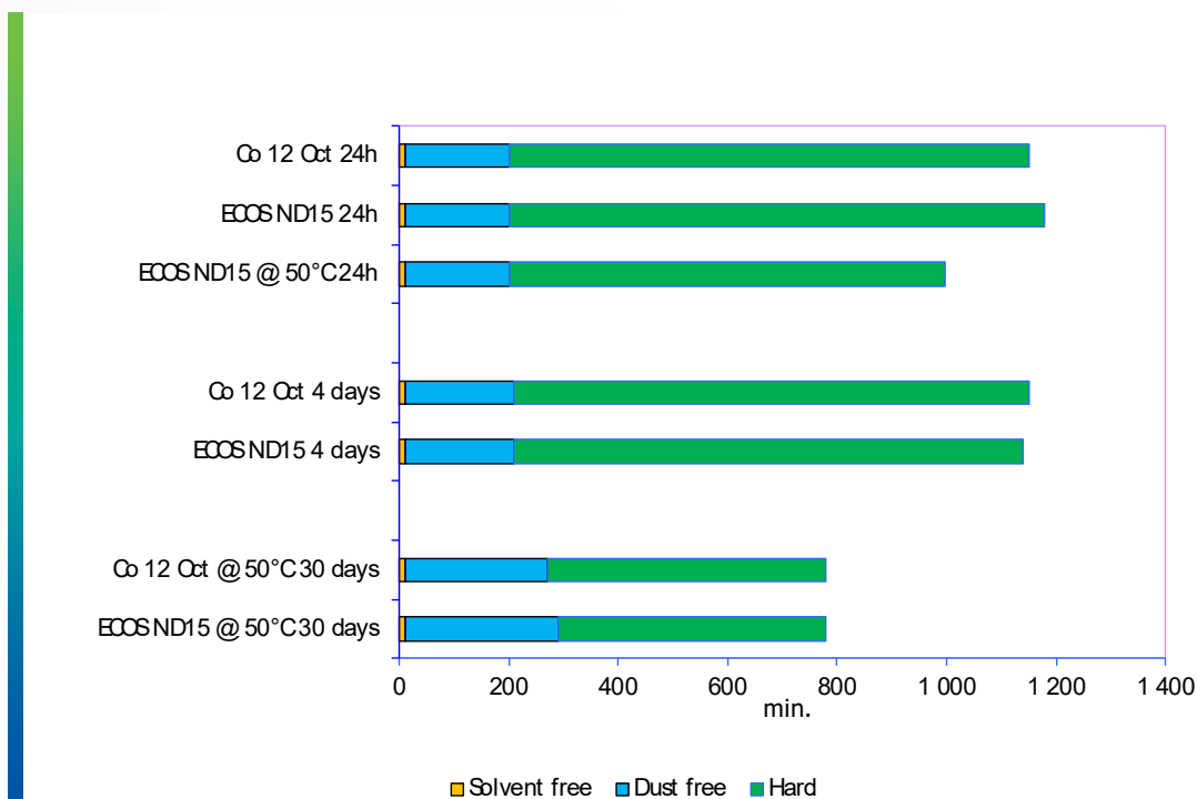
Graphic 1 : Drying time ECOS ND ® 15 - Long oil white gloss paint
